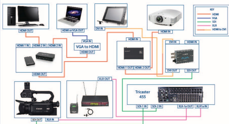
UC Berkeley 540 CORY HALL - A/V Signal Flow Diagram
